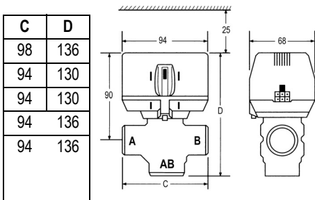
Fig. 1: Dimensions (mm)
