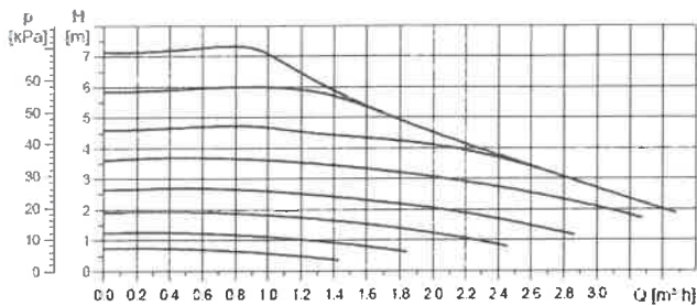
UPM2 25-70 180, 1 x 230 V, 50/60 Hz
