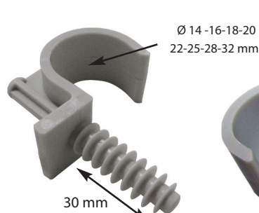
FIX-RING® Simple
