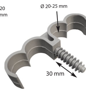
FIX-RING® Quadruple
