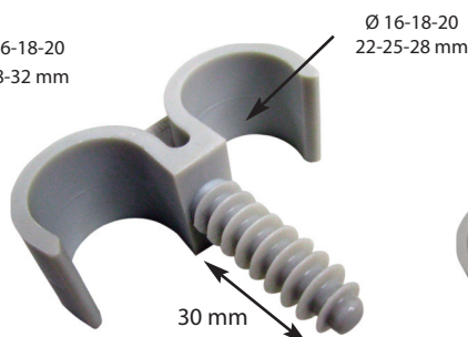
FIX-RING® Double
